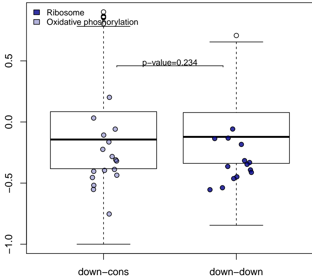
BOUND correlation
