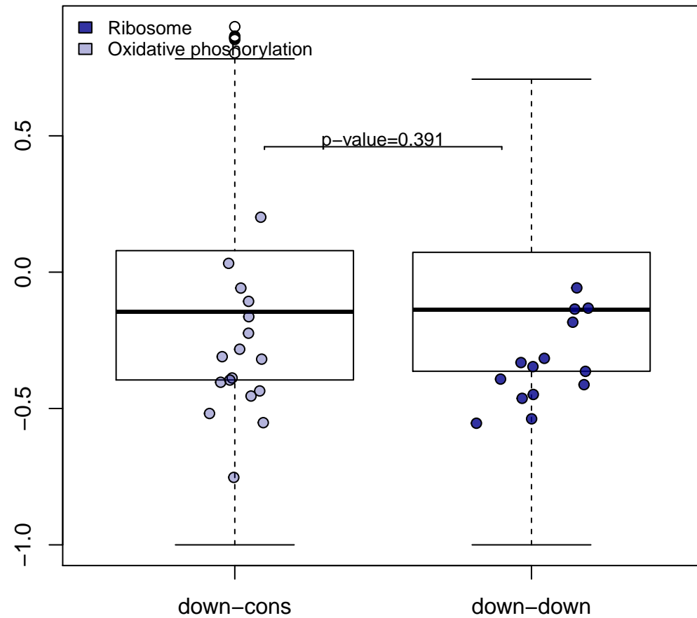
TOTAL correlation
